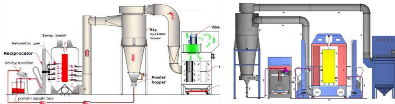
Powder spray booth system -Big cyclone serie
